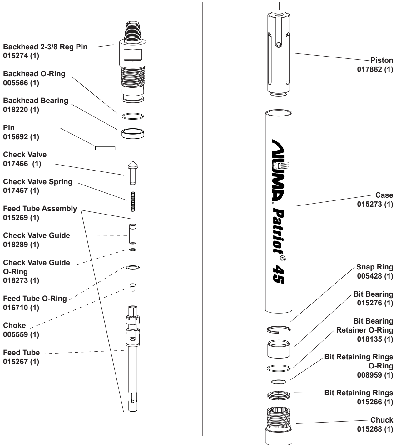
Hammer Assembly #017864 Figure 3-1
