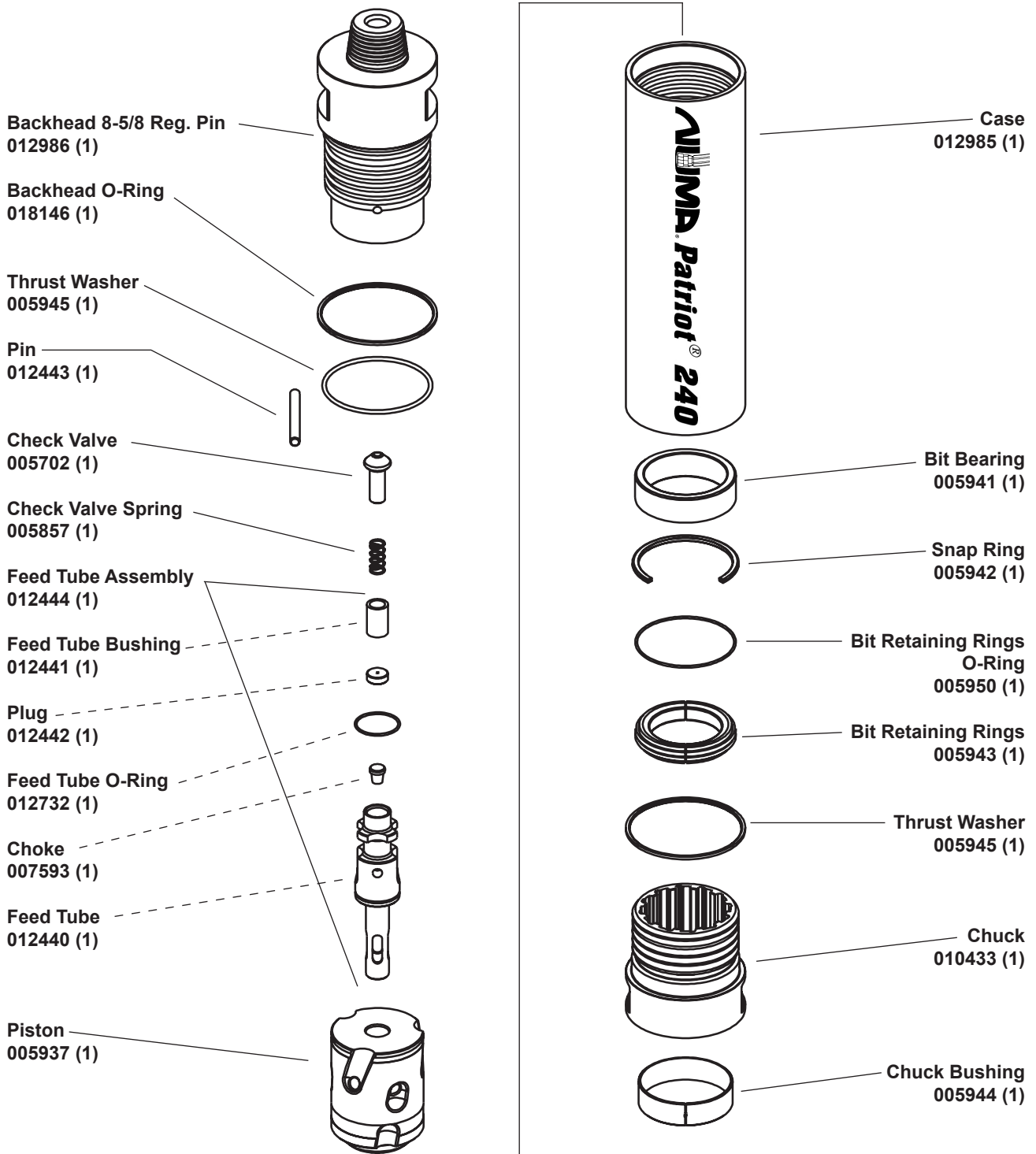
HAMMER ASSEMBLY #013987
