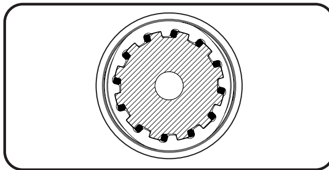
Drive Plate Positioning as Viewed from Top of Chuck Figure 2-3
