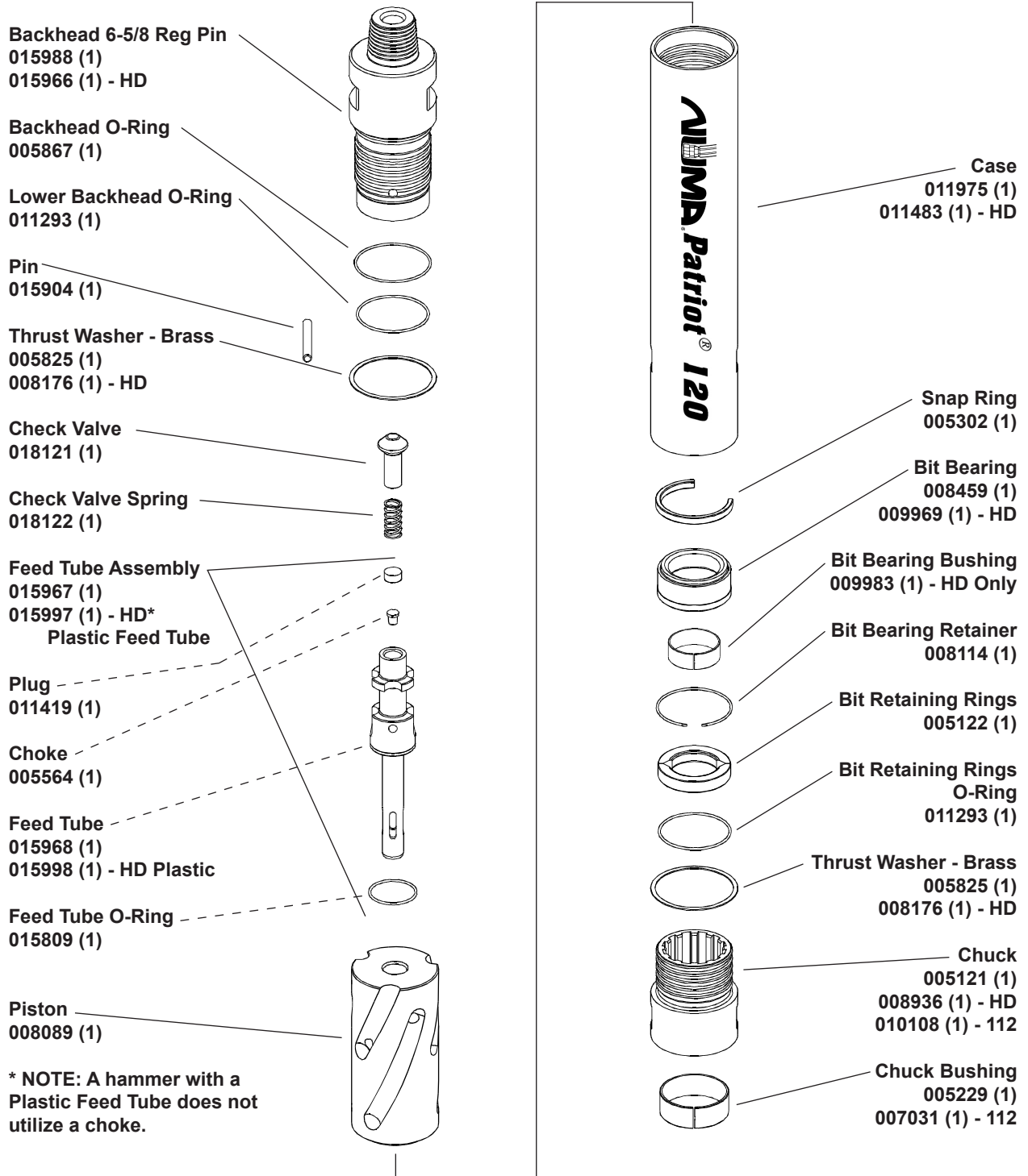
Hammer Assembly #015989 / HD #015977 / 112 Bits #015976
