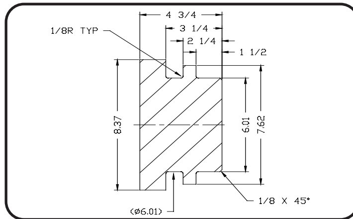
P120/120HD Bearing Spacer/Press Plate Figure 2-1
