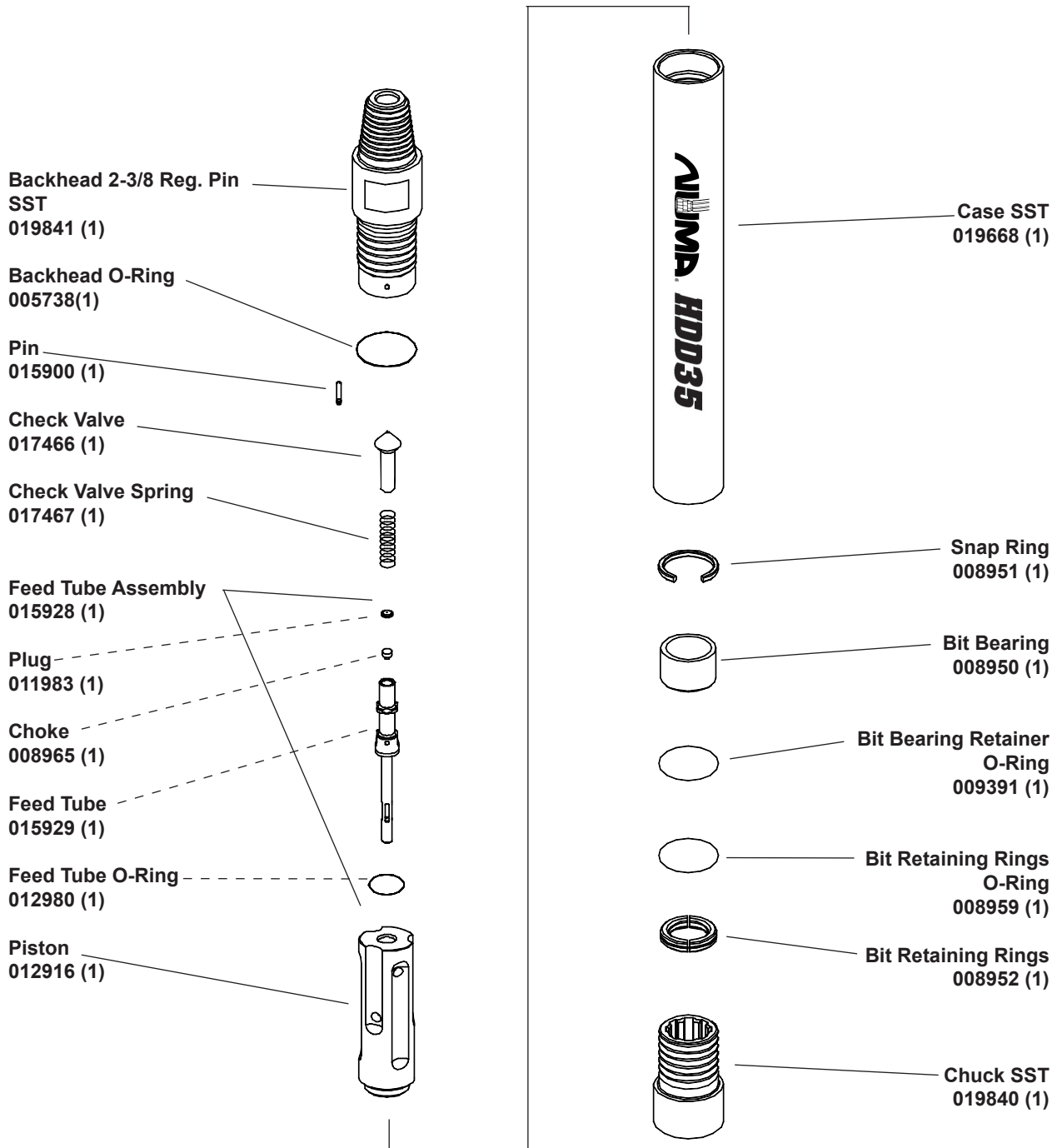
Hammer Assembly #020168 Figure 3-1
